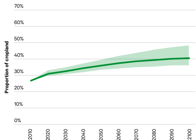
Figure 10b. Proportion of global rice crop area experiencing damaging hot spells
