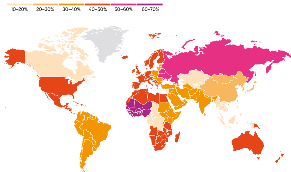
Figure 9b. Proportion of regional cropland exposed to severe drought, in 2050
