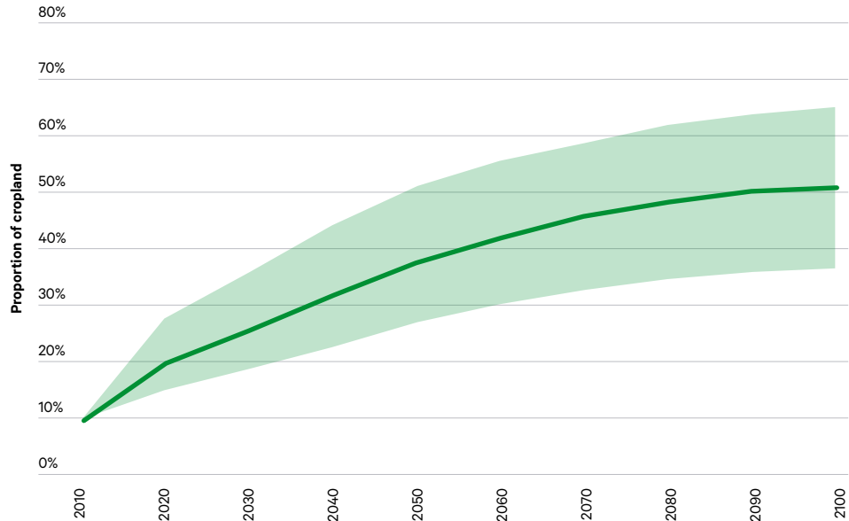
Figure 9a. Proportion of global cropland experiencing severe drought of three months or more per year
