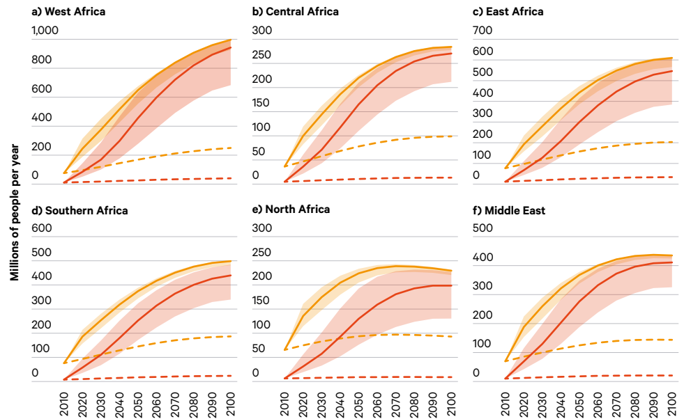
Figure 5. Populations within African regions and the Middle East experiencing heatwaves and major heatwaves
